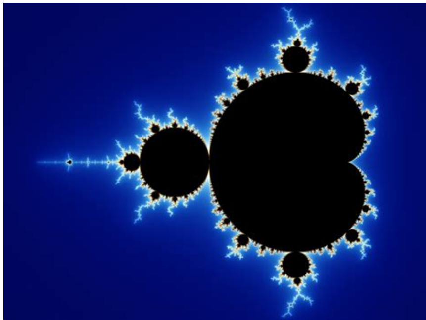
The Mandelbrot set
